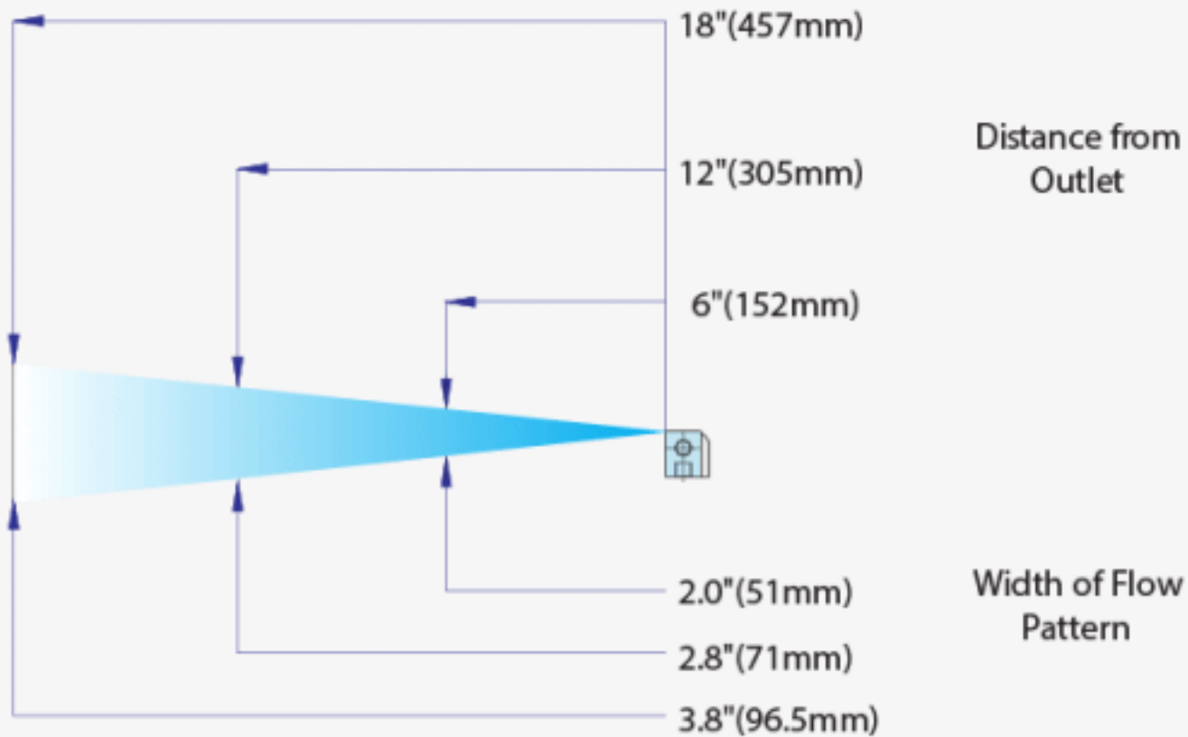
CONCENTRATED KNIFE EDGE AIR STREAM OF STANDARD AIR BLADE™ AIR KNIFE
